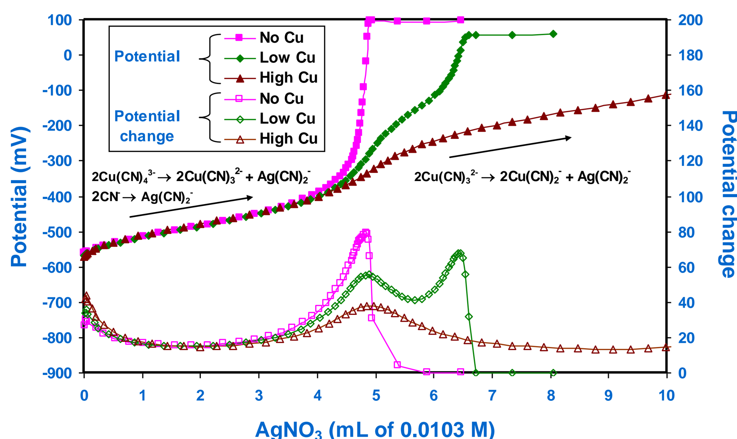
Figure 1: Potentiometric titration of 20 mL samples containing 250 mg/L NaCN; low Cu – 100 mg/L Cu as \text{Cu}(\text{CN})_3^{2-} , high Cu – 500 mg/L Cu as \text{Cu}(\text{CN})_3^{2-} .
